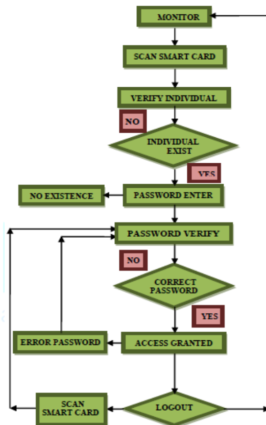
Fig.1 OTP Authentication
